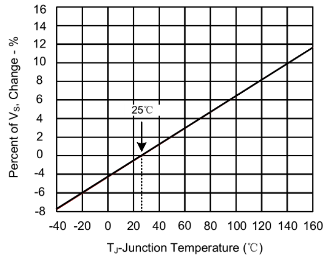
Figure 2. Normalized V_S Change versus Junction Temperature
