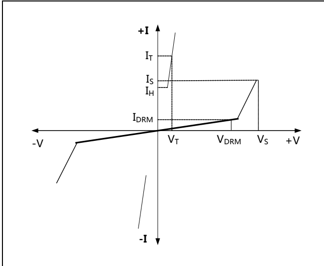
Figure 1. V/I Characteristics
