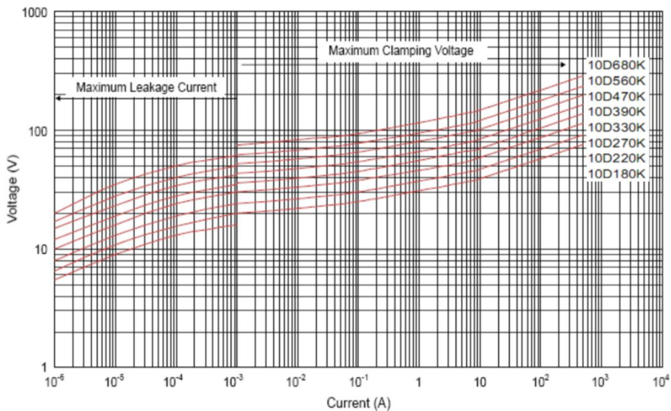
10D180K to 10D680K
