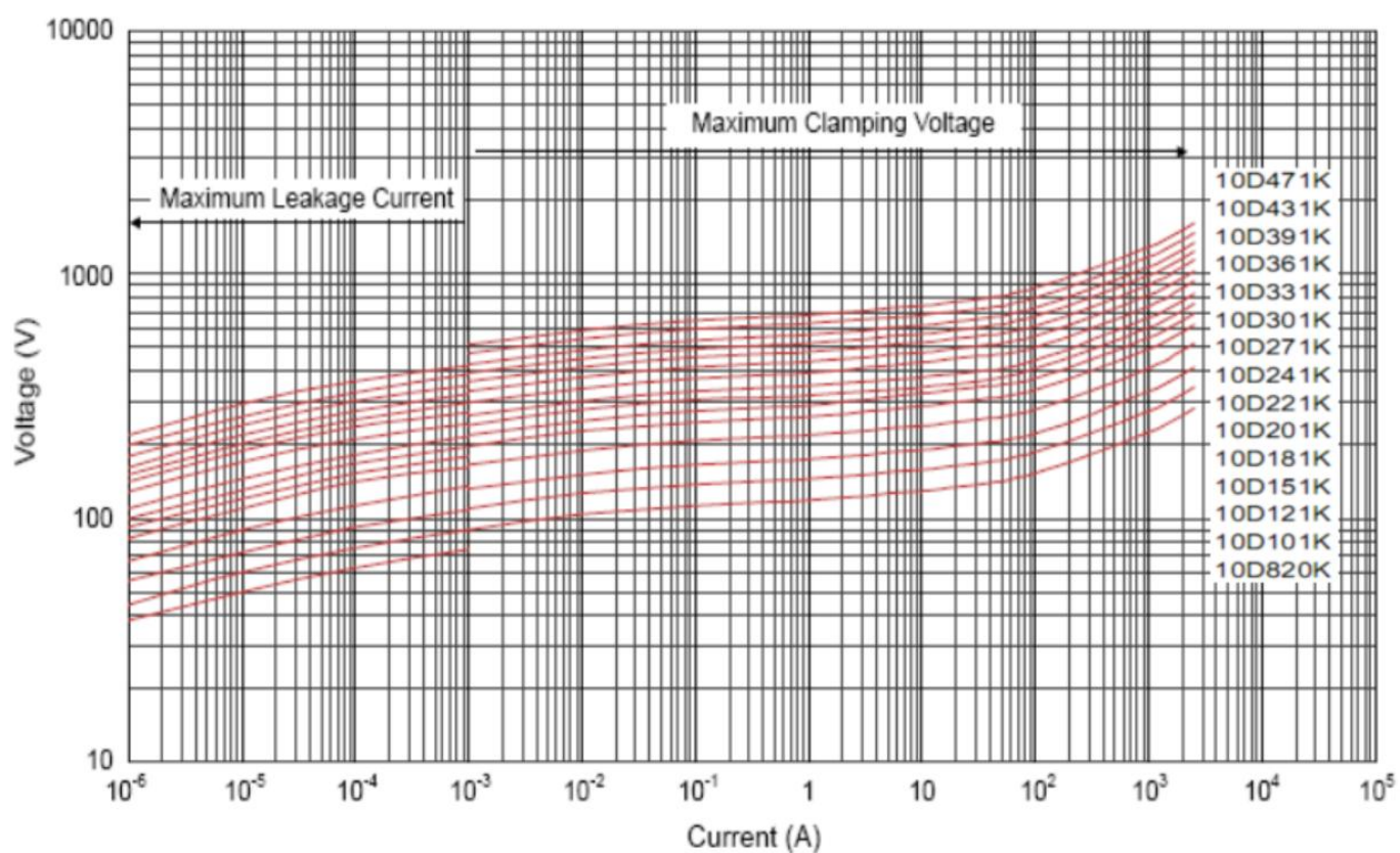
10D820K to 10D471K
