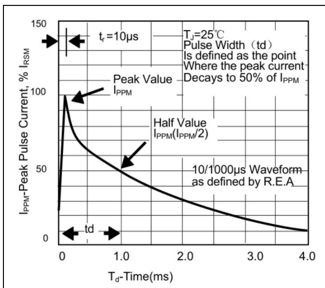
Figure 3. Pulse Waveform
